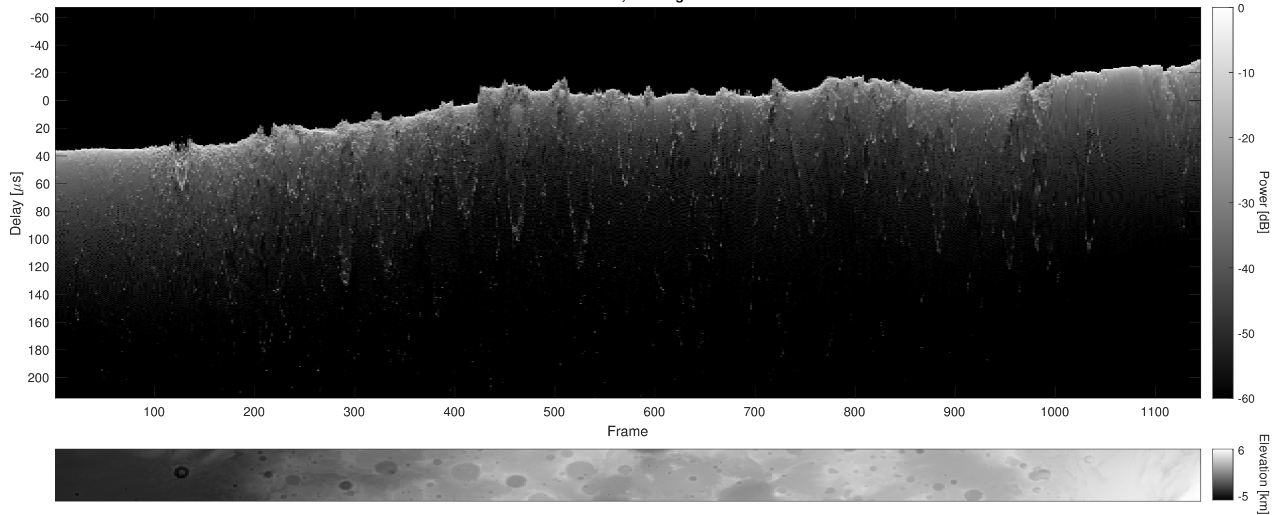
Orbit 13226, Cluttergram
