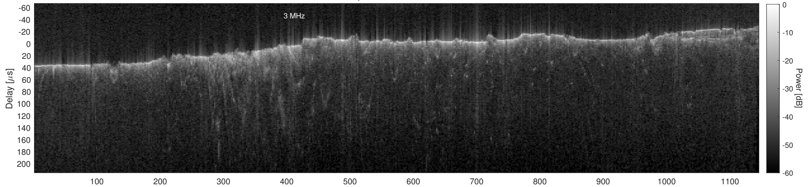
Orbit 13226, Cluttergram
