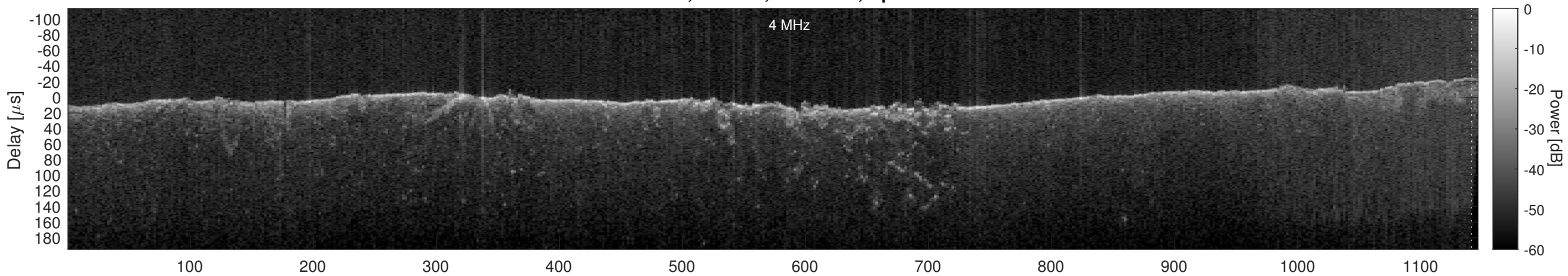
Orbit 13231, Cluttergram
