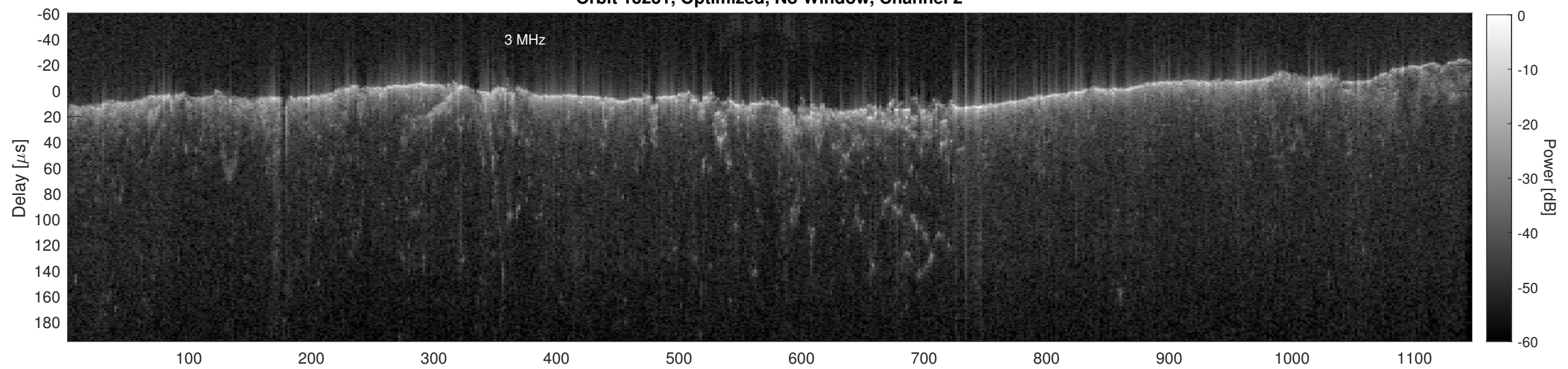
Orbit 13231, Cluttergram
