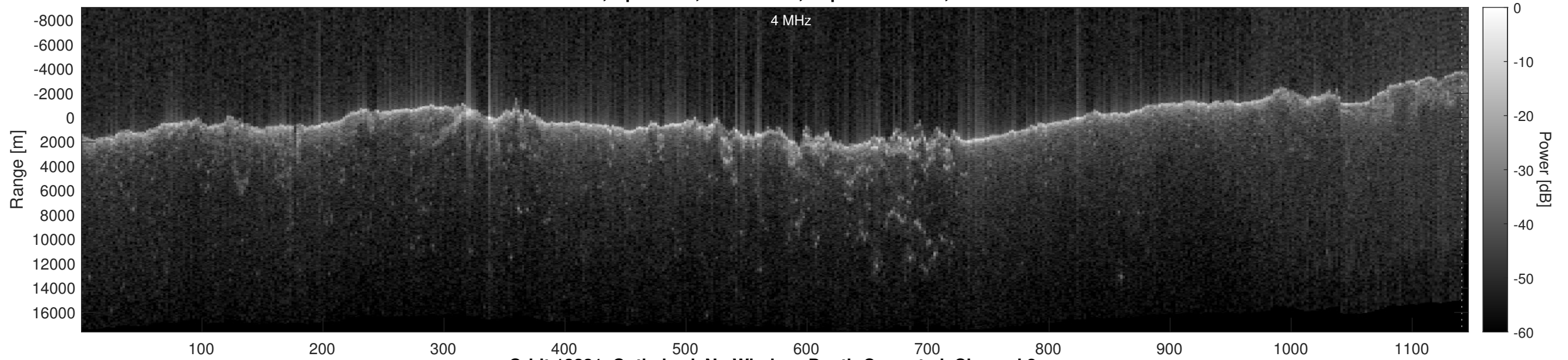
Orbit 13231, Optimized, No Window, Depth-Corrected, Channel 2
