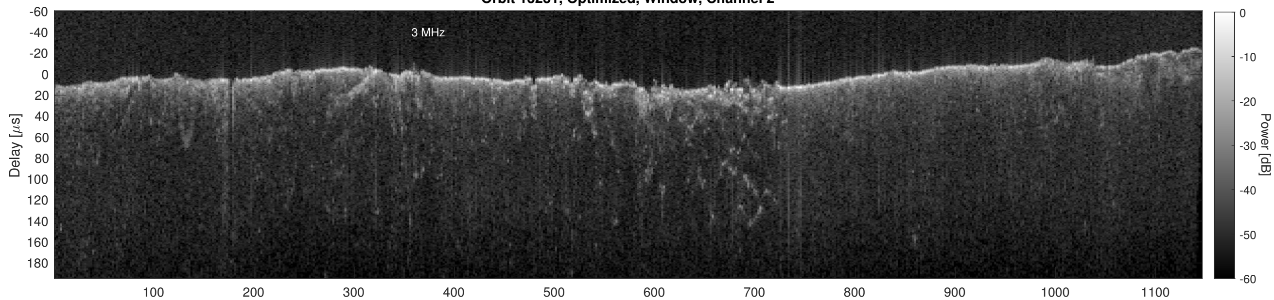
Orbit 13231, Cluttergram
