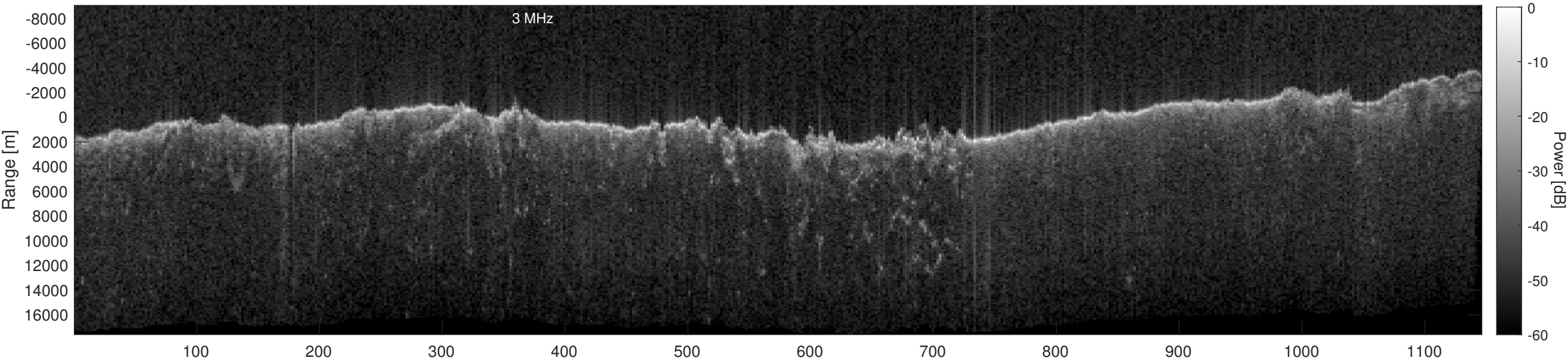
Orbit 13231, Depth-Corrected Cluttergram
