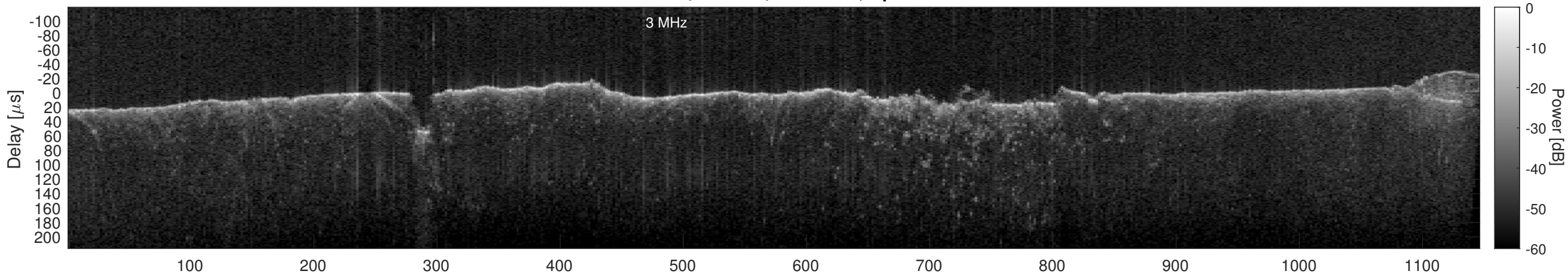
Orbit 13232, Cluttergram
