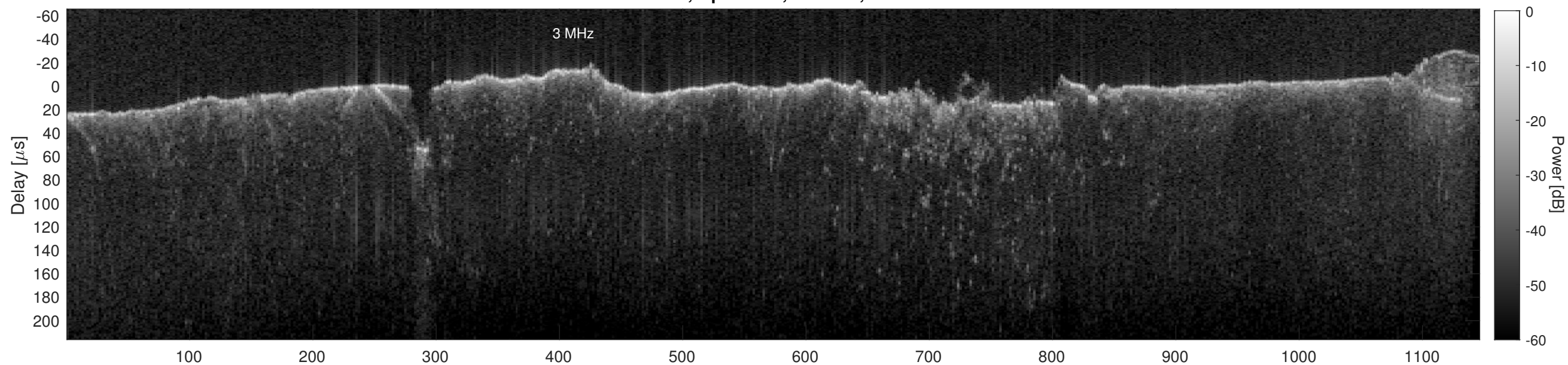
Orbit 13232, Cluttergram
