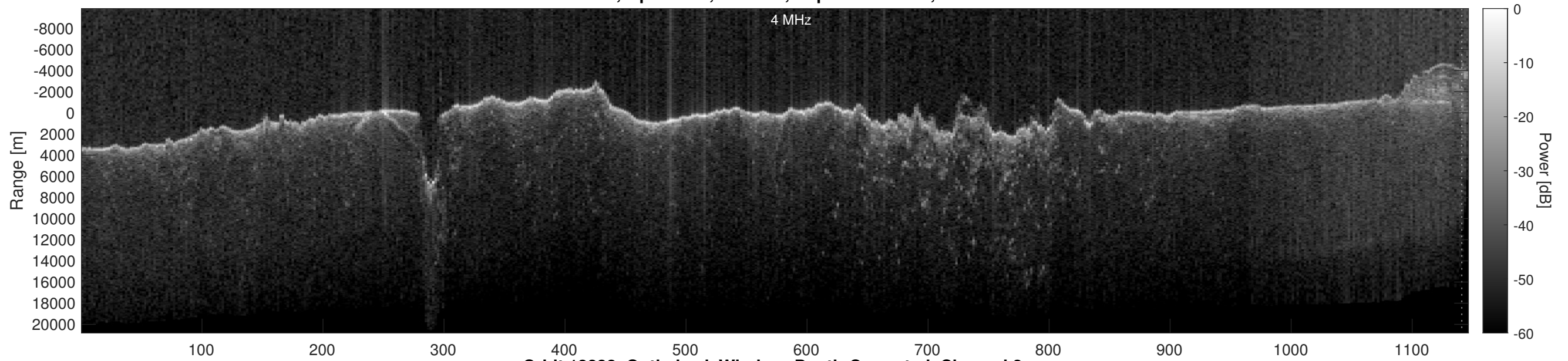
Orbit 13232, Optimized, Window, Depth-Corrected, Channel 2
