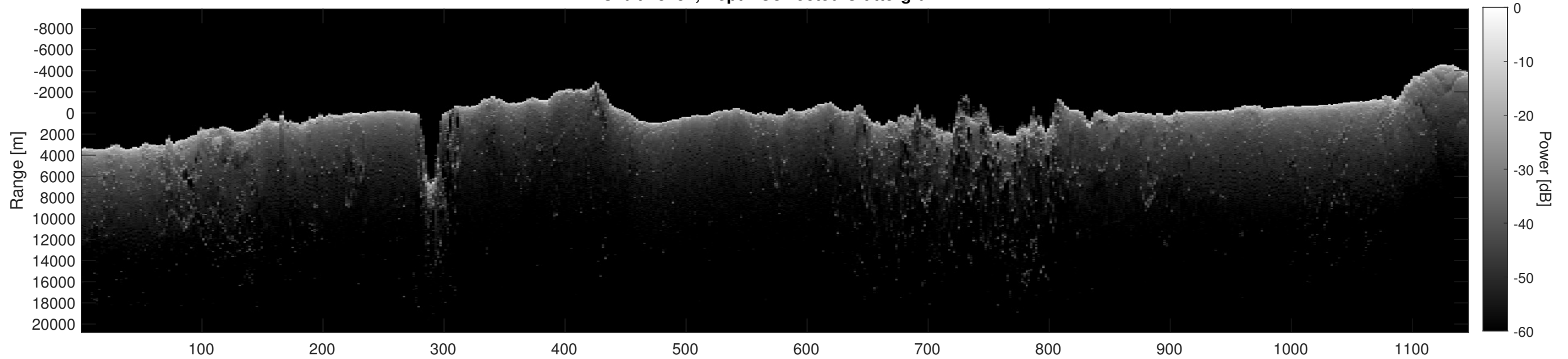
Orbit 13232, Depth-Corrected Cluttergram
