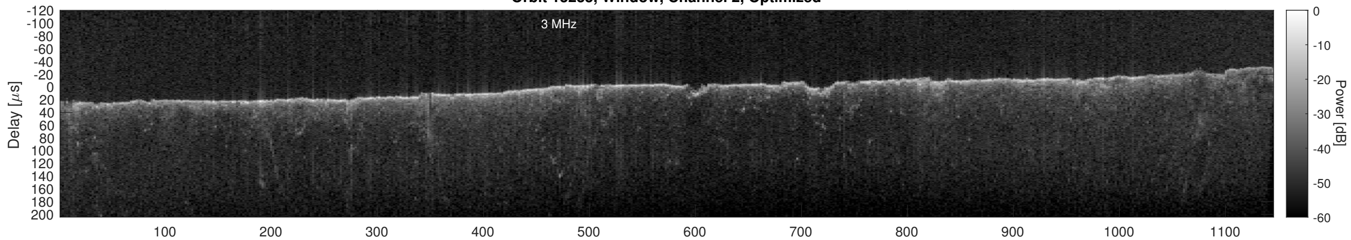
Orbit 13235, Cluttergram
