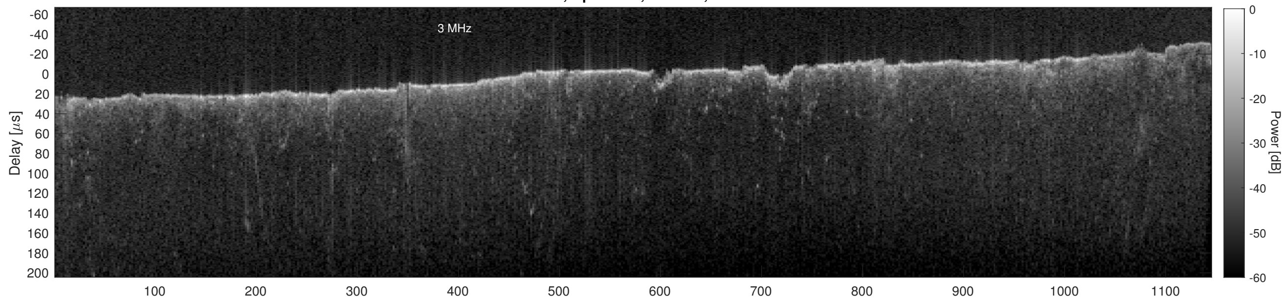
Orbit 13235, Cluttergram
