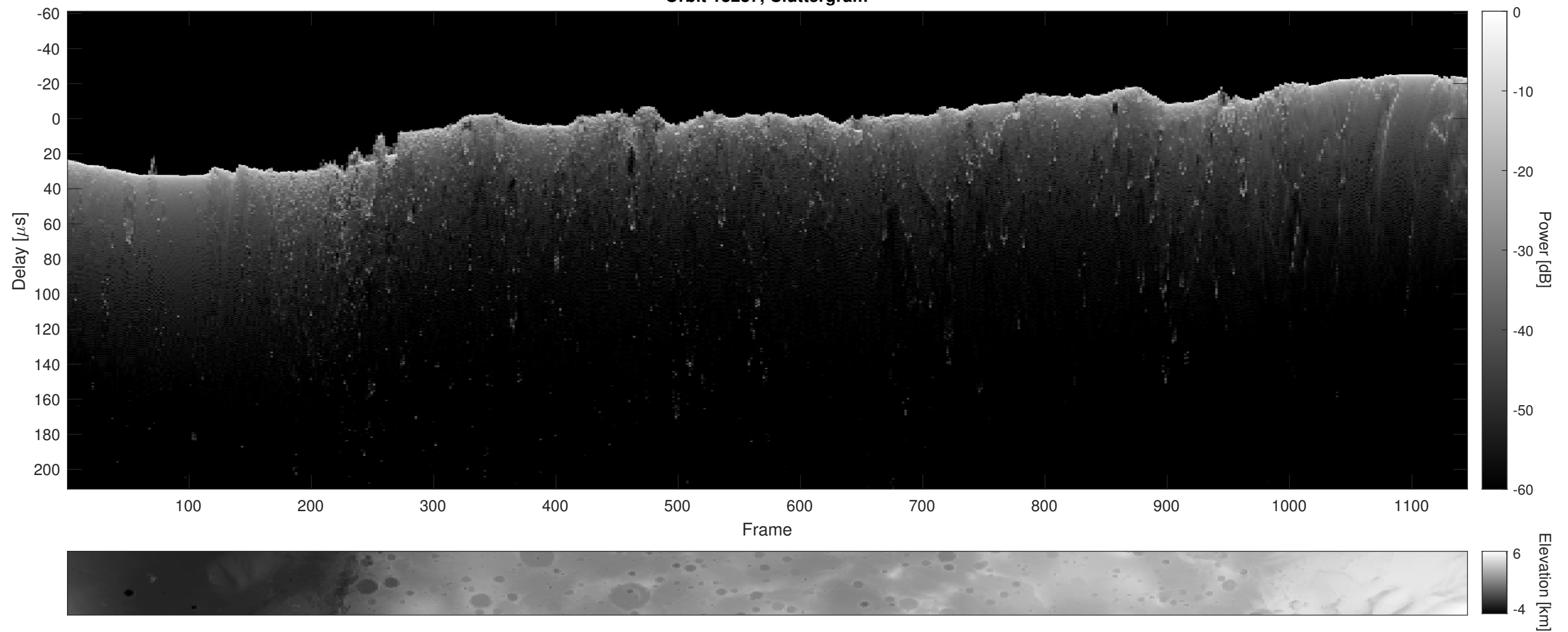
Orbit 13237, Cluttergram
