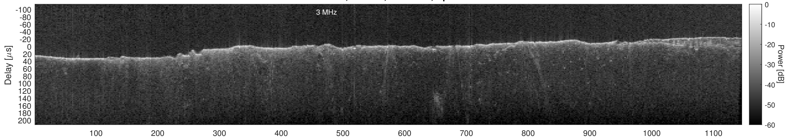
Orbit 13237, Cluttergram
