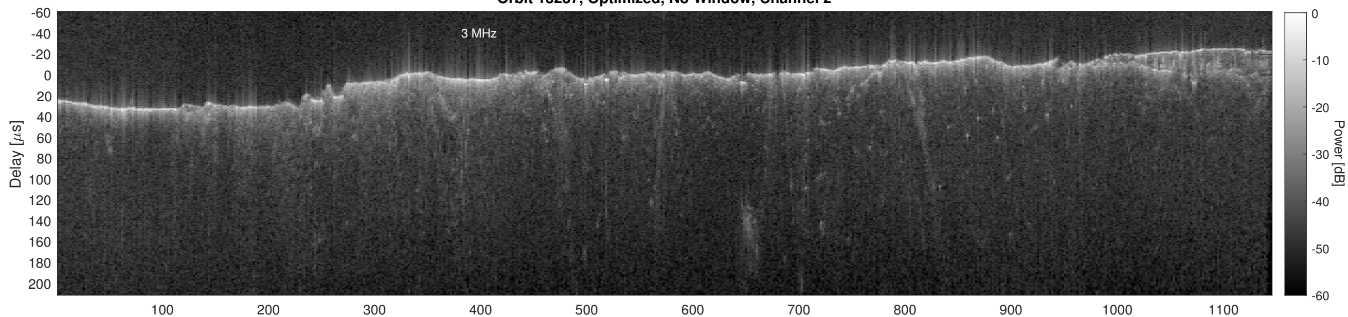
Orbit 13237, Cluttergram
