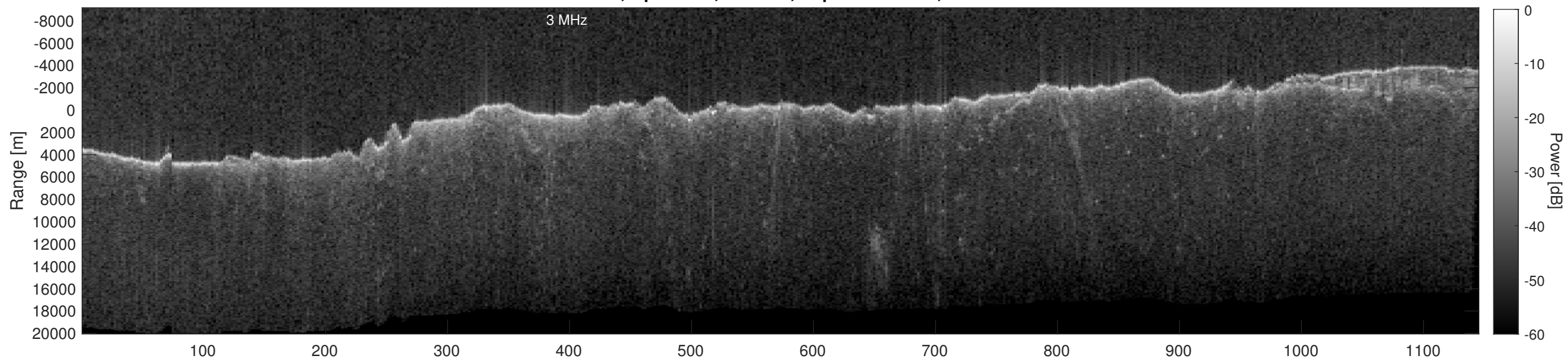
Orbit 13237, Depth-Corrected Cluttergram
