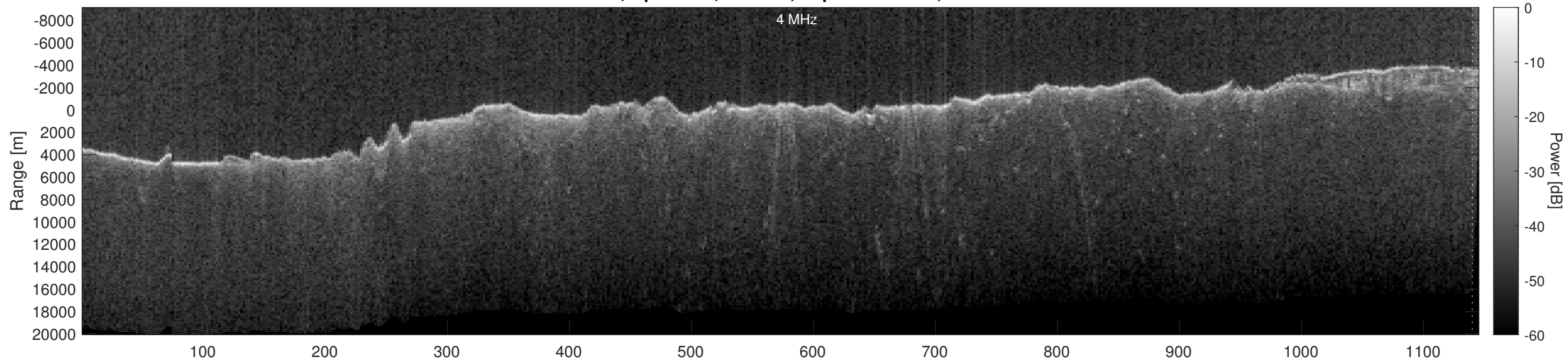
Orbit 13237, Optimized, Window, Depth-Corrected, Channel 2
