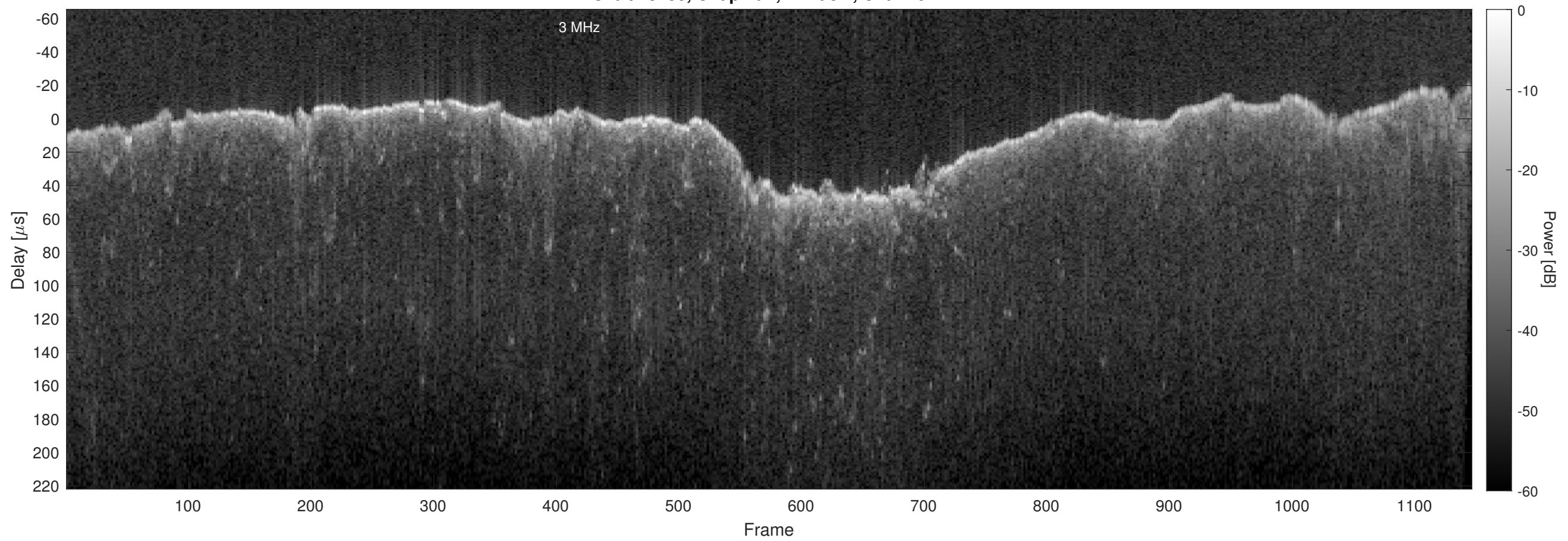
Orbit 13238, Chapman, Window, Channel 2
