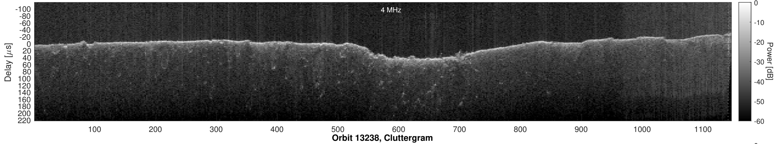
Orbit 13238, Window, Channel 1, Optimized
