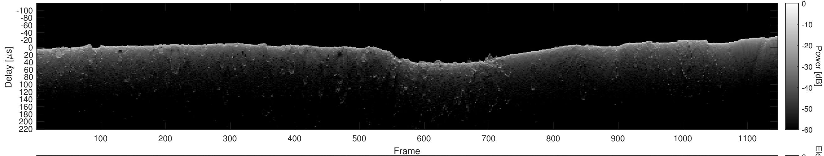
Orbit 13238, Cluttergram
