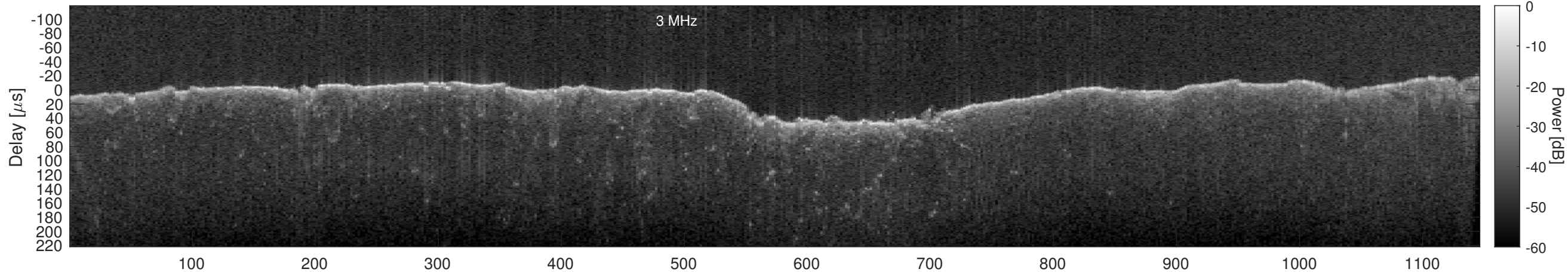
Orbit 13238, Window, Channel 2, Chapman
