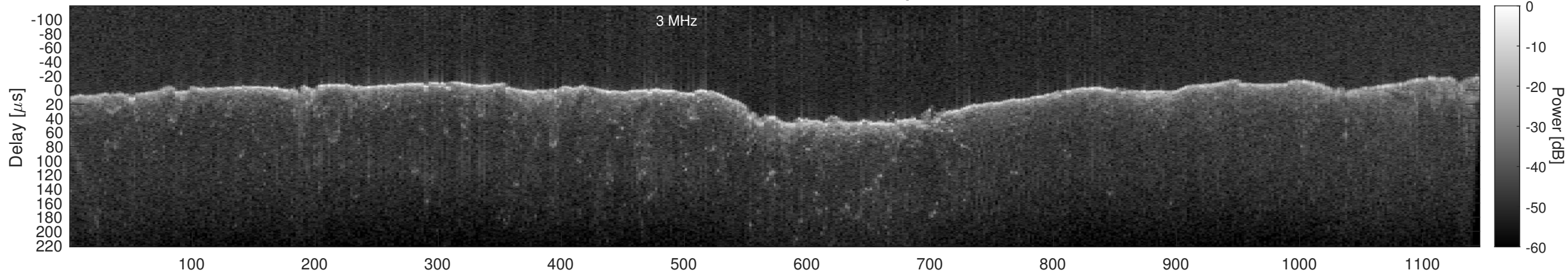
Orbit 13238, Window, Channel 2, Optimized
