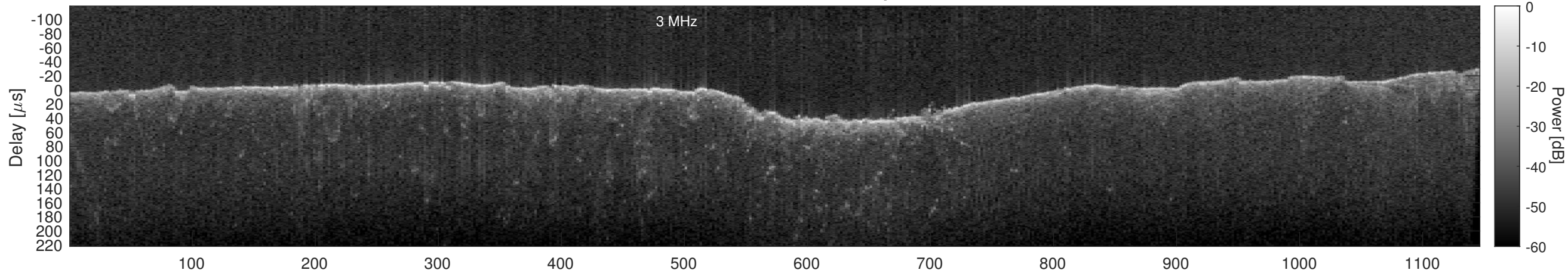
Orbit 13238, Cluttergram
