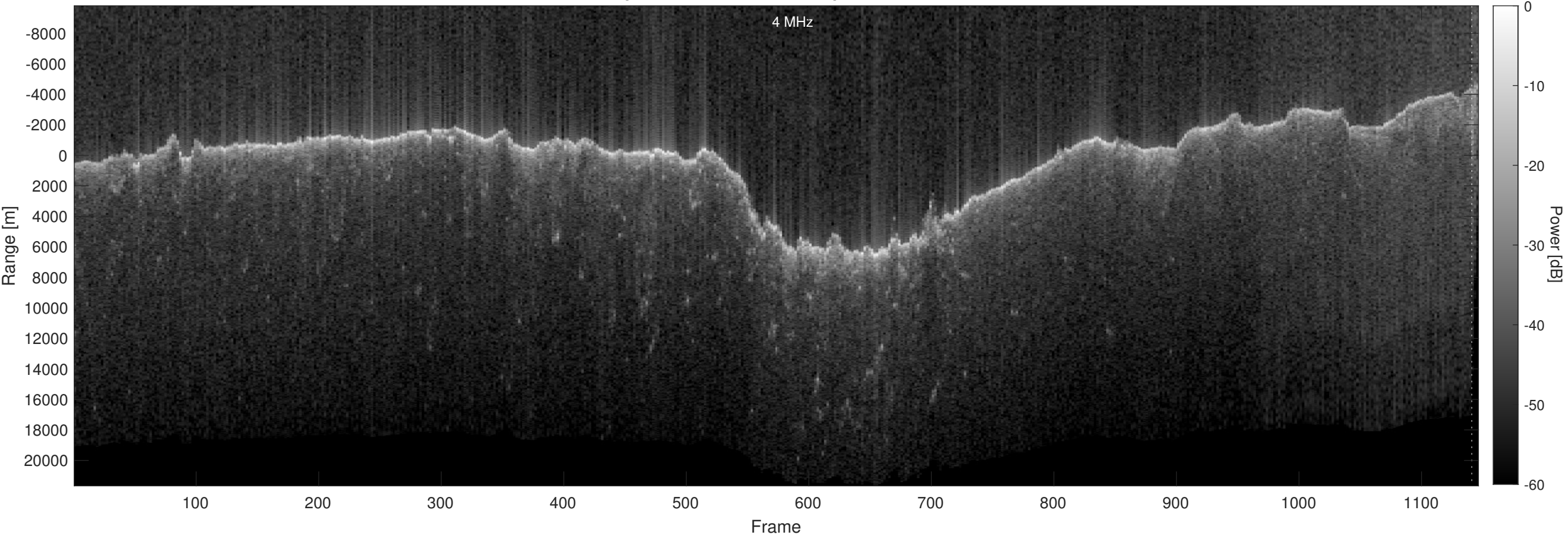
Orbit 13238, Optimized, No Window, Depth-Corrected, Channel 2
