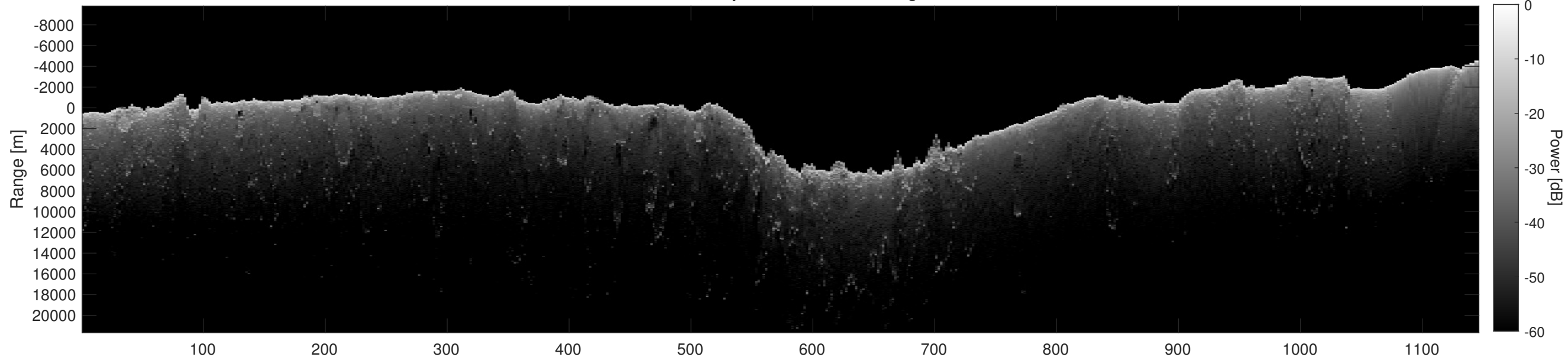
Orbit 13238, Depth-Corrected Cluttergram
