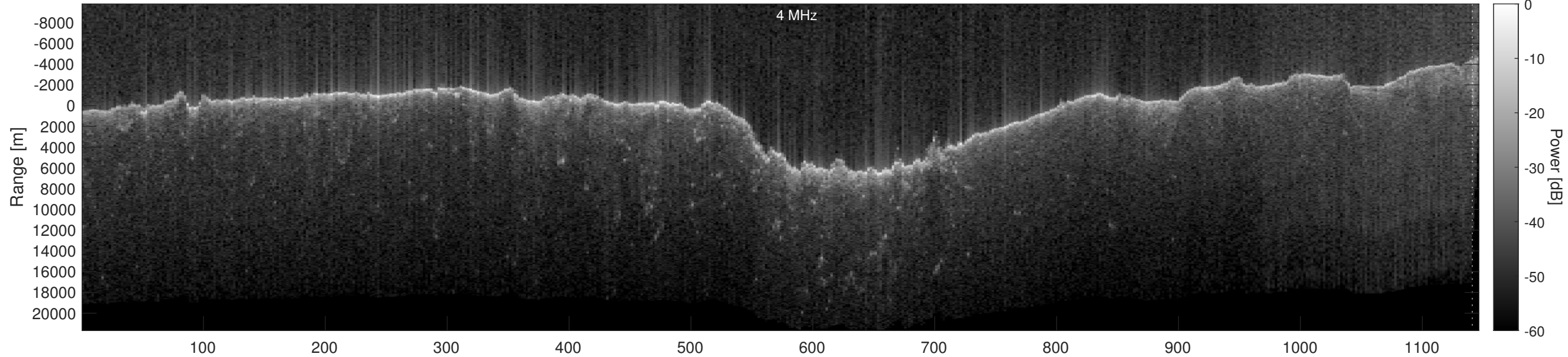
Orbit 13238, Optimized, No Window, Depth-Corrected, Channel 2
