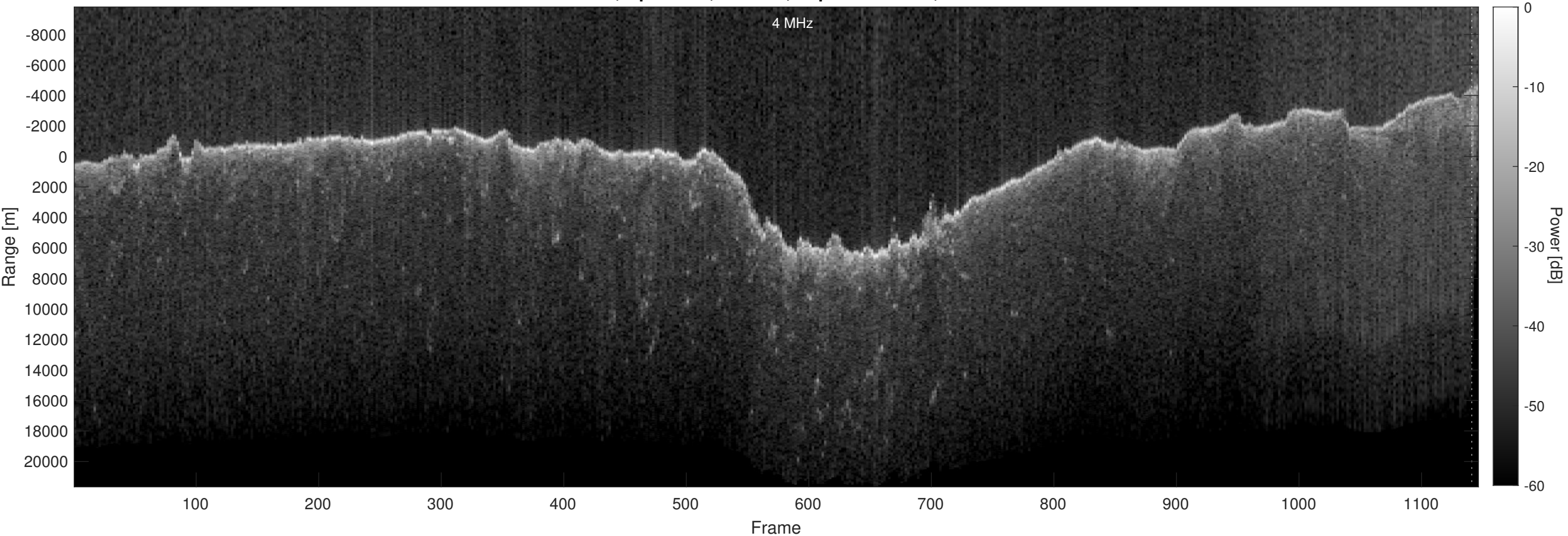
Orbit 13238, Optimized, Window, Depth-Corrected, Channel 2
