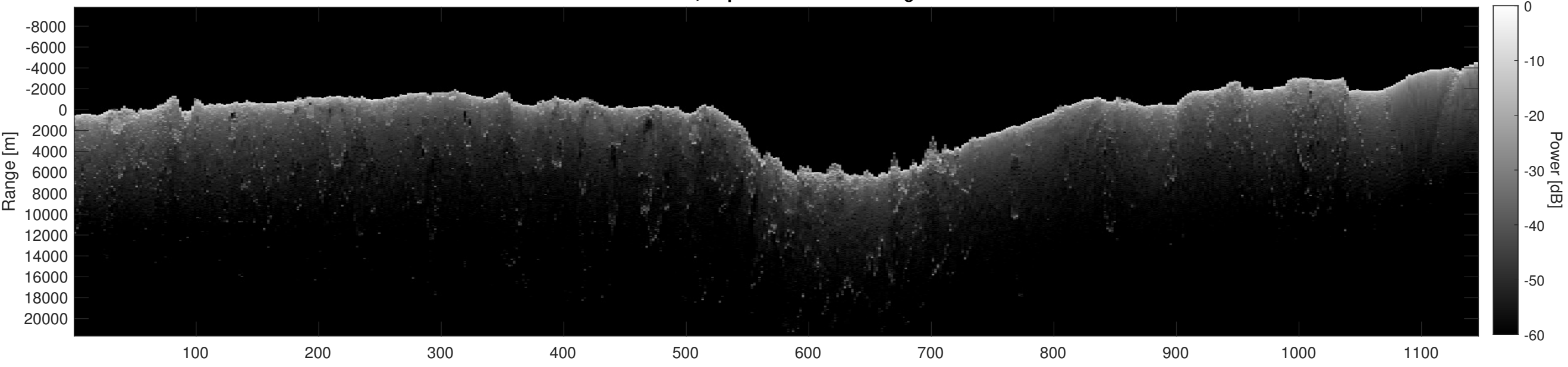
Orbit 13238, Depth-Corrected Cluttergram
