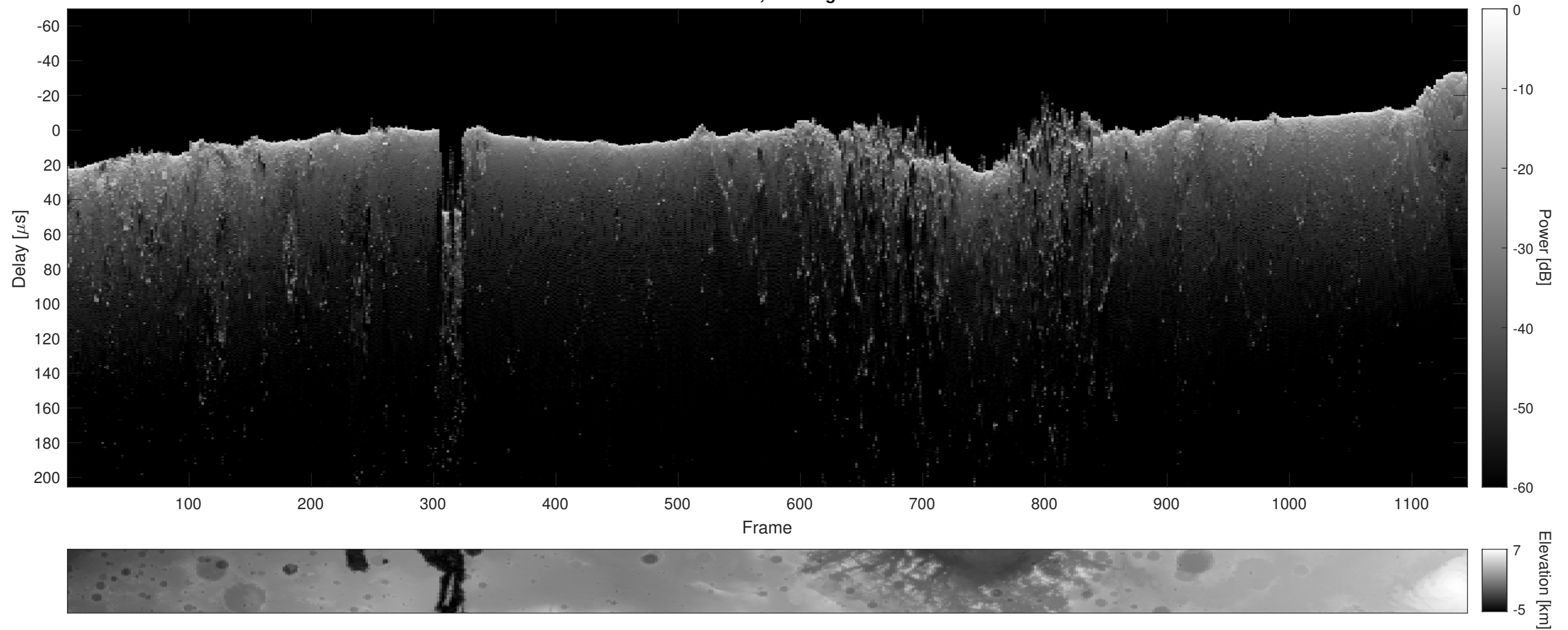
Orbit 13239, Cluttergram
