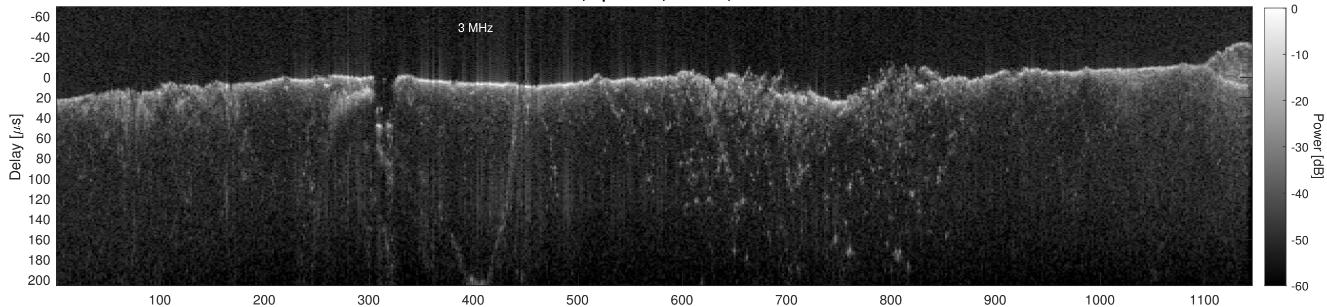
Orbit 13239, Cluttergram
