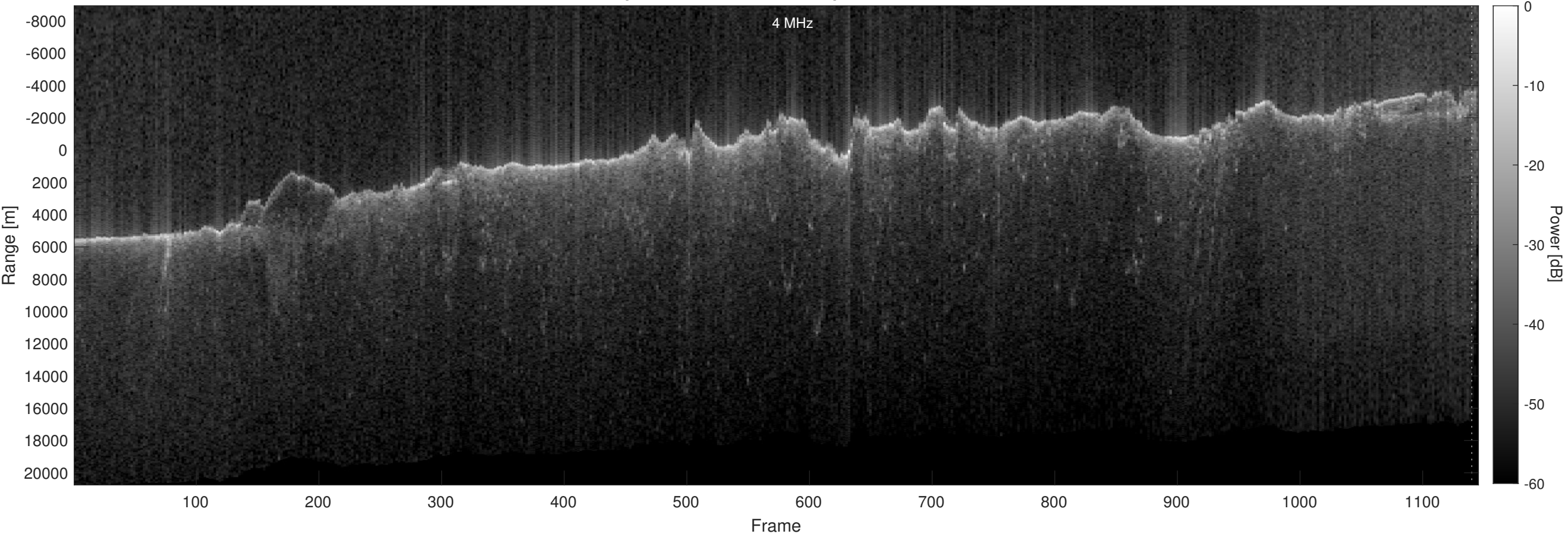
Orbit 13240, Optimized, No Window, Depth-Corrected, Channel 2
