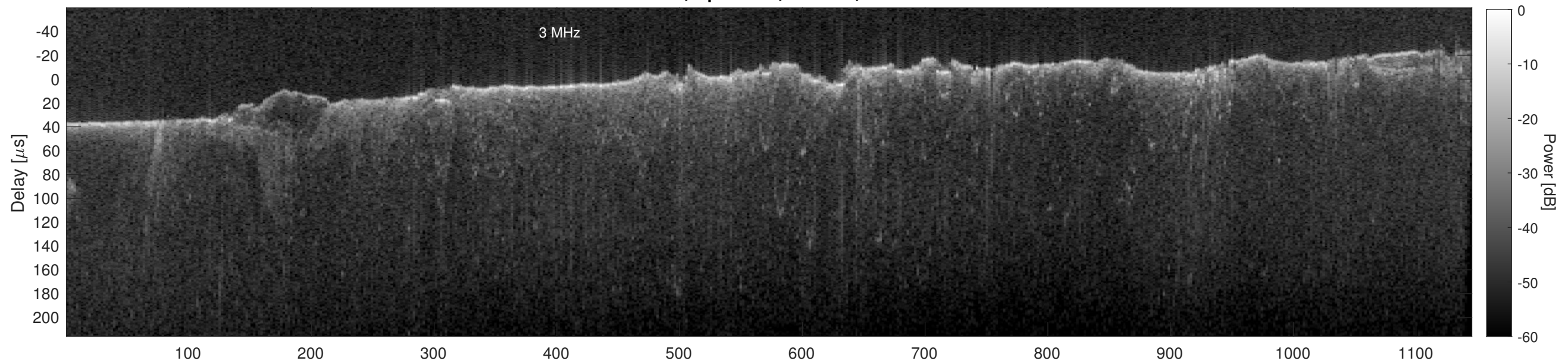
Orbit 13240, Cluttergram
