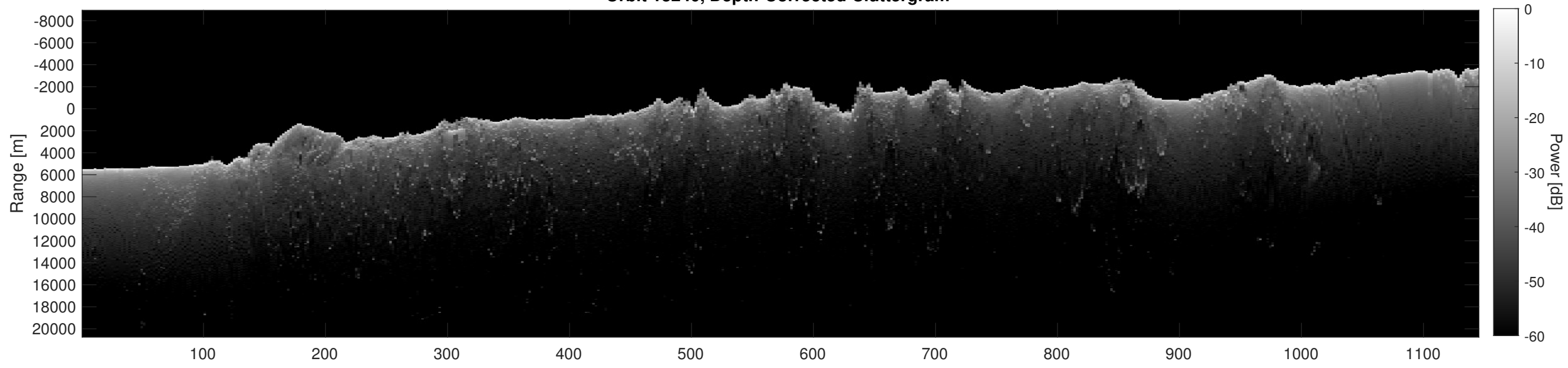
Orbit 13240, Depth-Corrected Cluttergram
