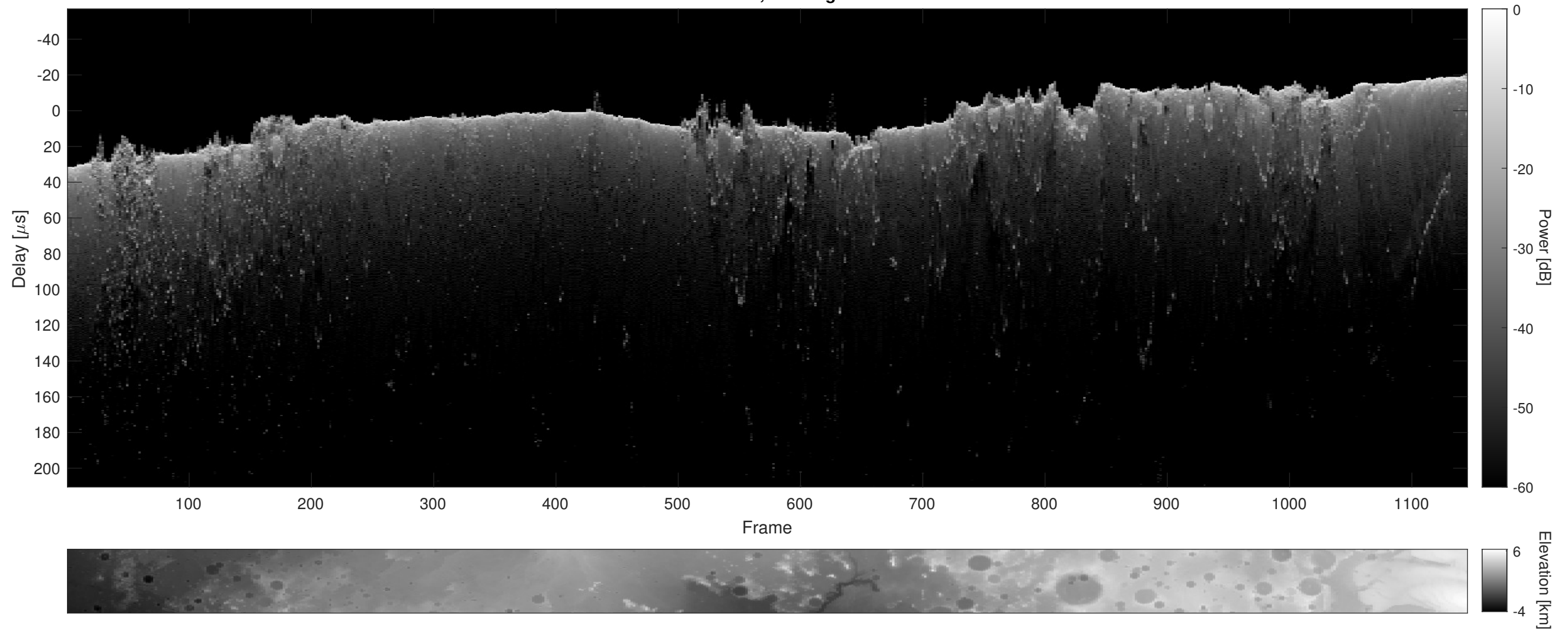
Orbit 13241, Cluttergram
