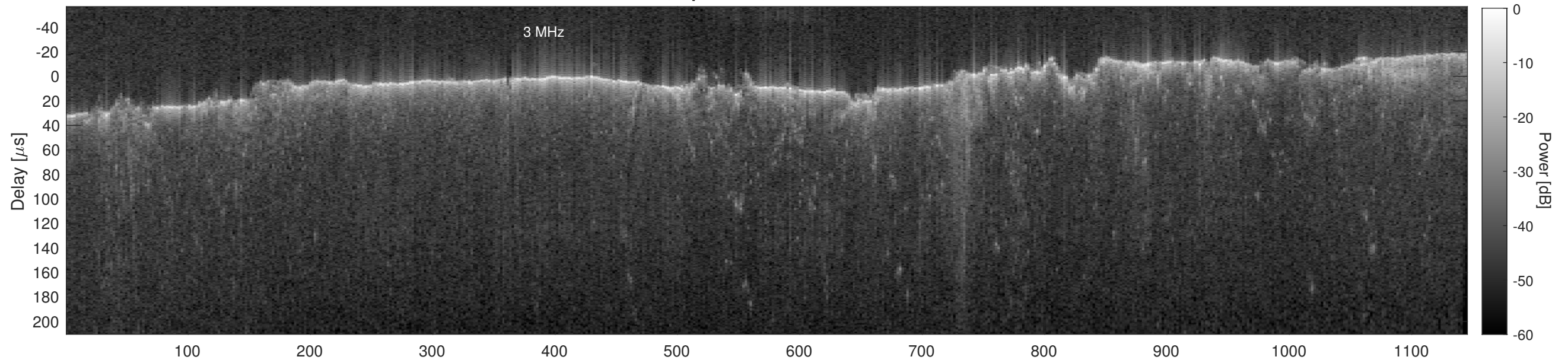
Orbit 13241, Cluttergram
