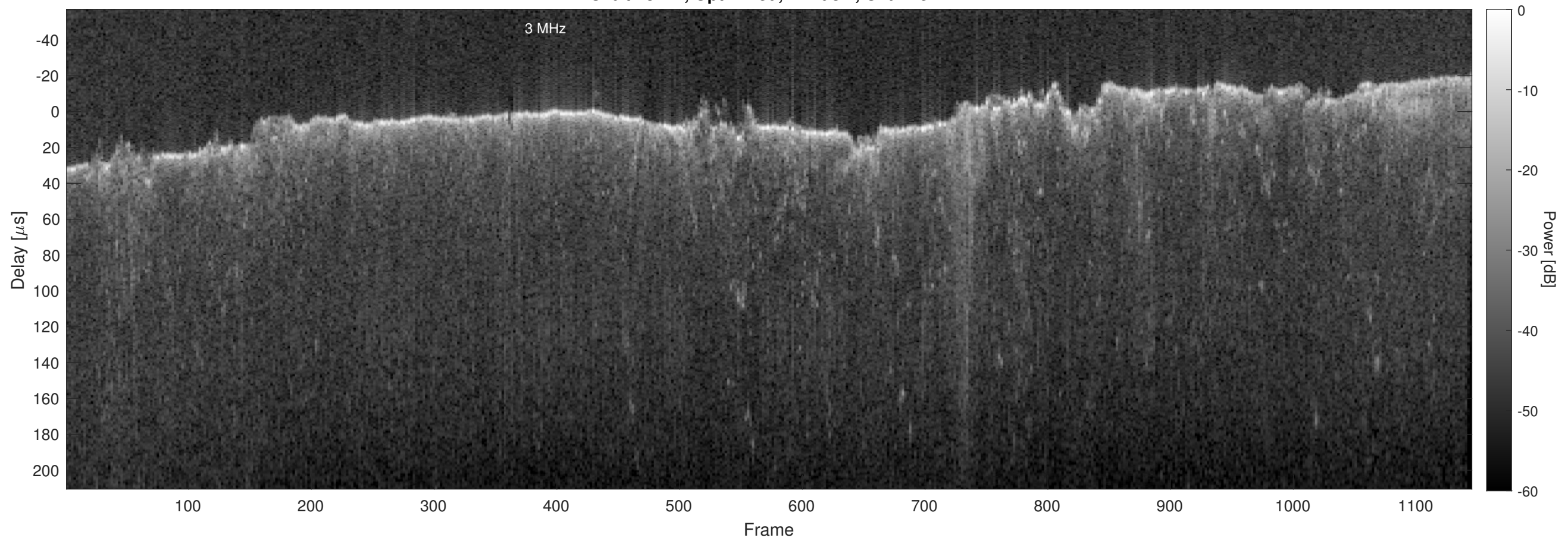
Orbit 13241, Optimized, Window, Channel 2
