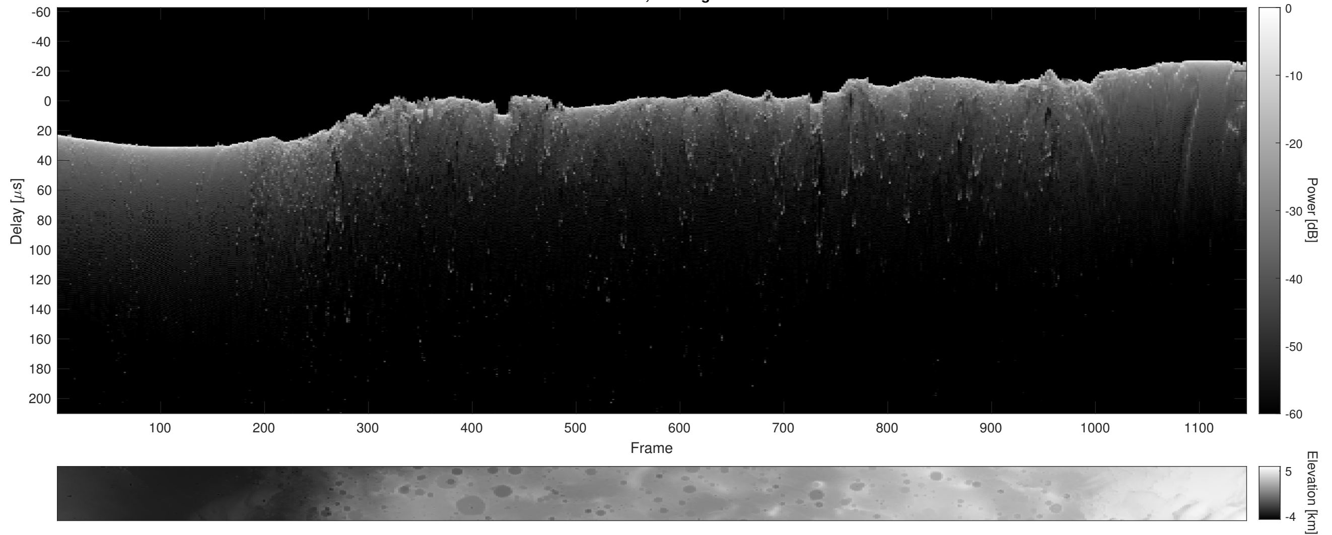
Orbit 13244, Cluttergram
