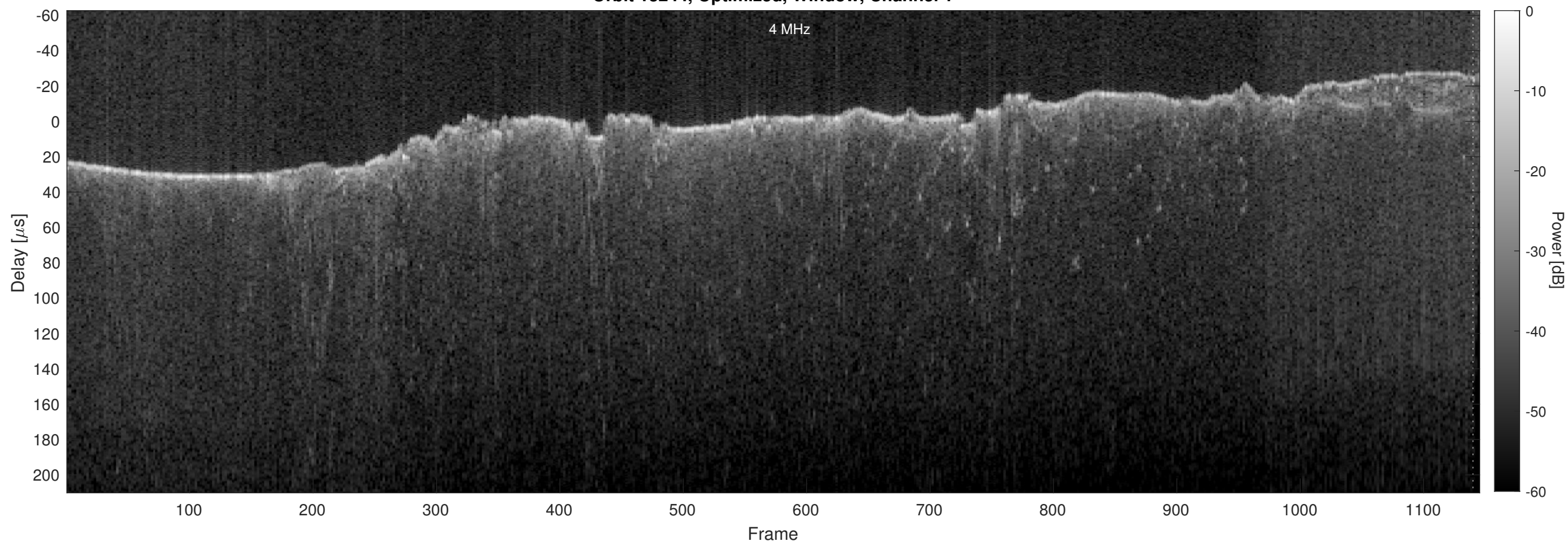
Orbit 13244, Optimized, Window, Channel 2
