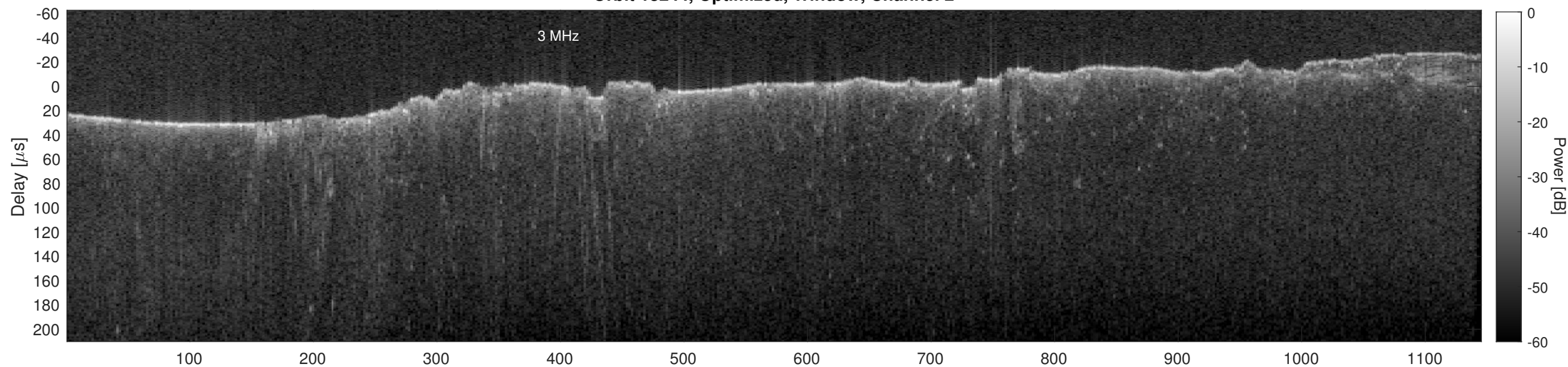
Orbit 13244, Cluttergram
