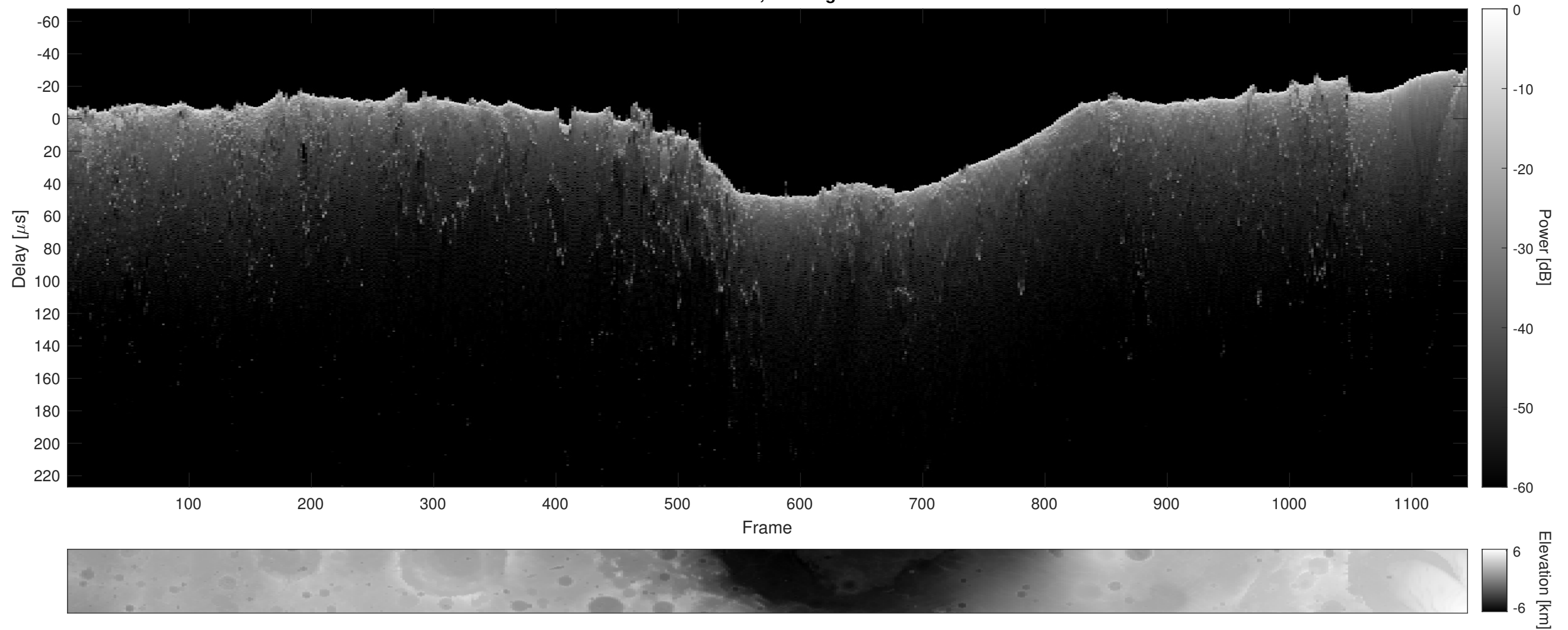
Orbit 13245, Cluttergram
