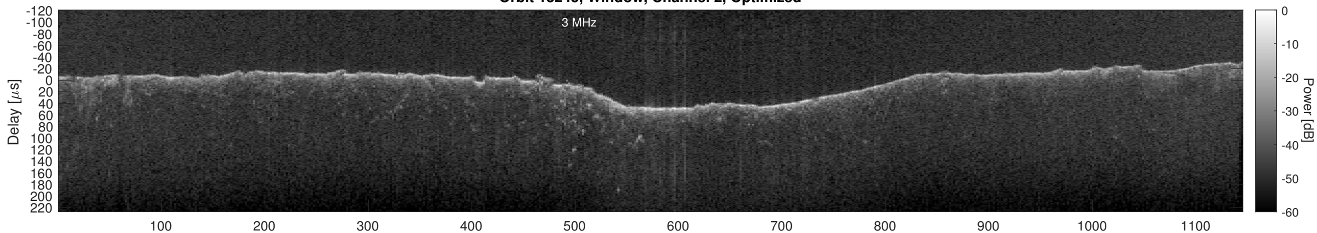
Orbit 13245, Cluttergram
