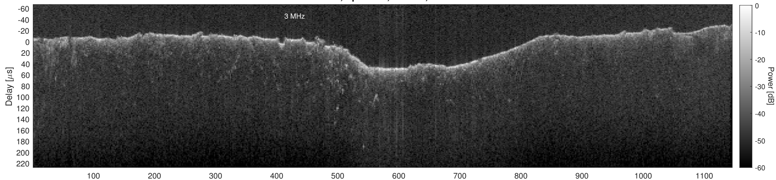
Orbit 13245, Cluttergram
