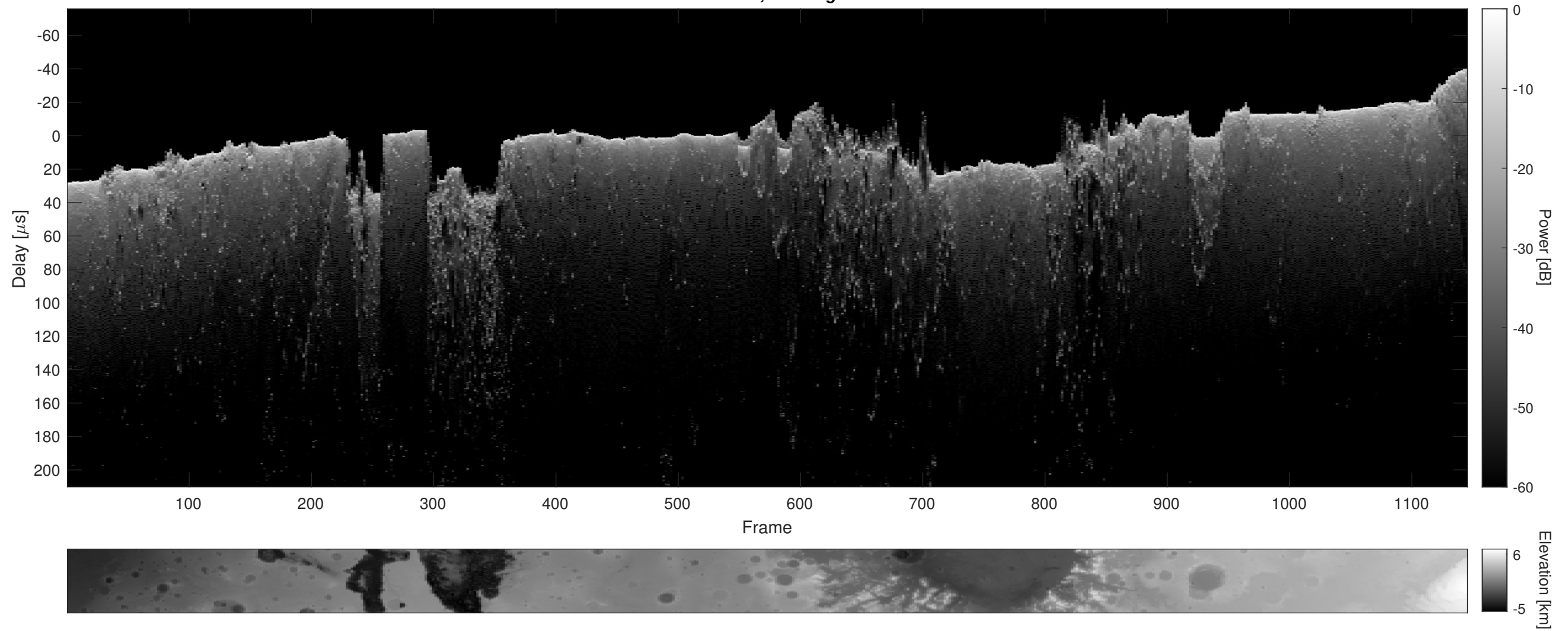
Orbit 13246, Cluttergram
