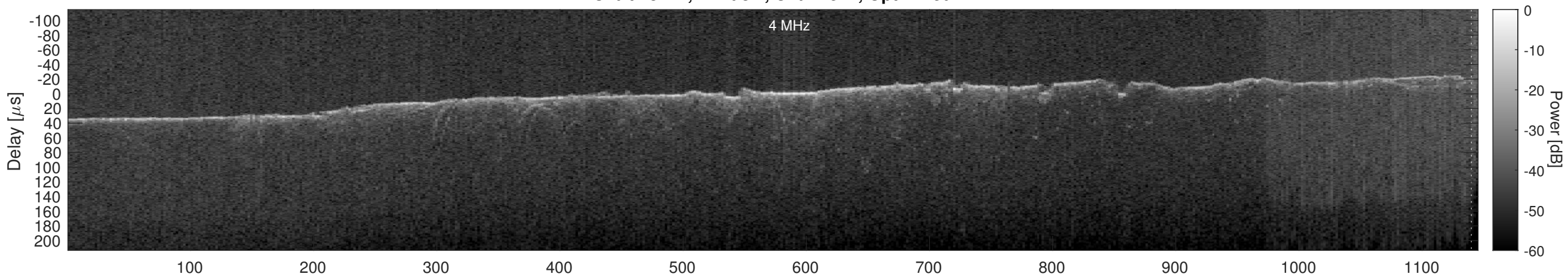
Orbit 13247, Cluttergram
