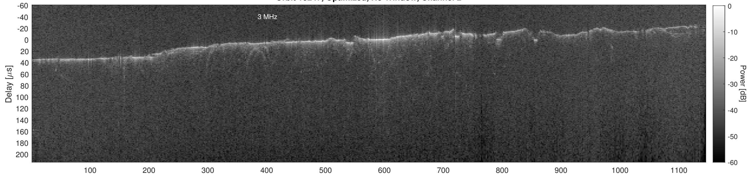
Orbit 13247, Cluttergram
