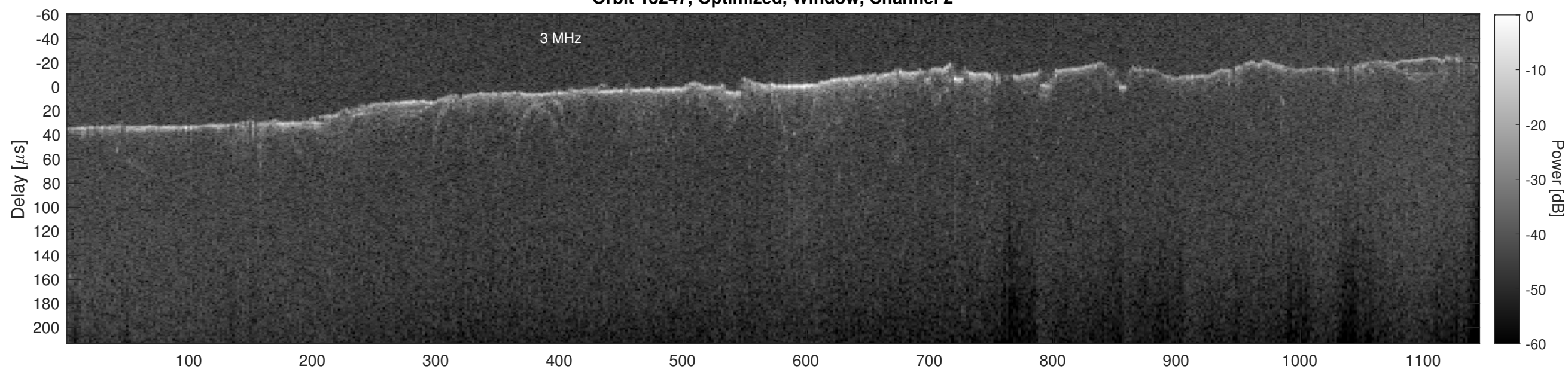
Orbit 13247, Cluttergram
