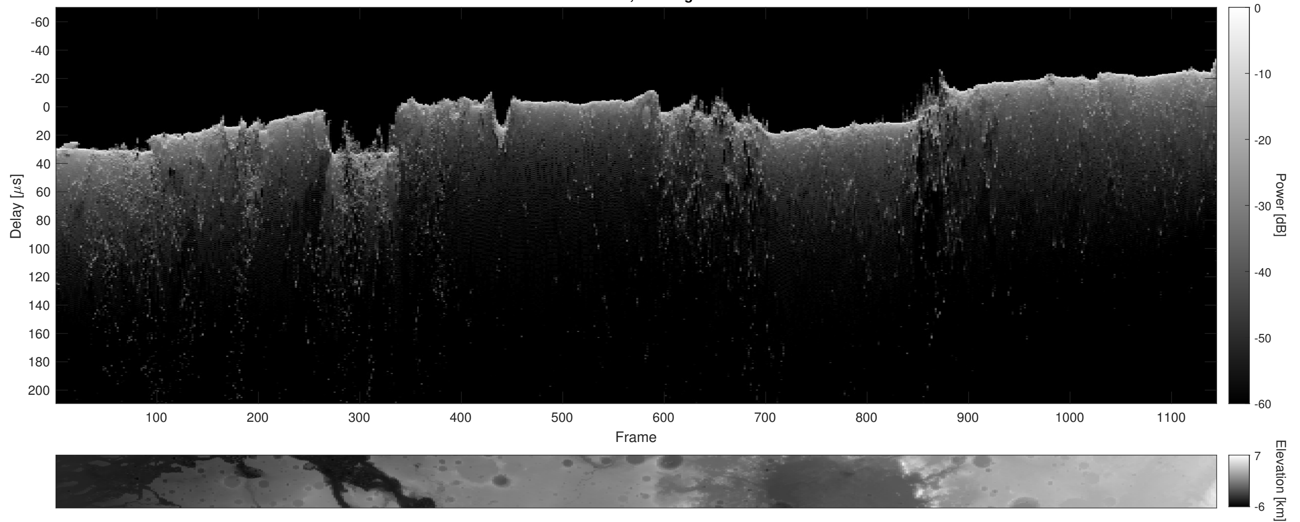
Orbit 13260, Cluttergram
