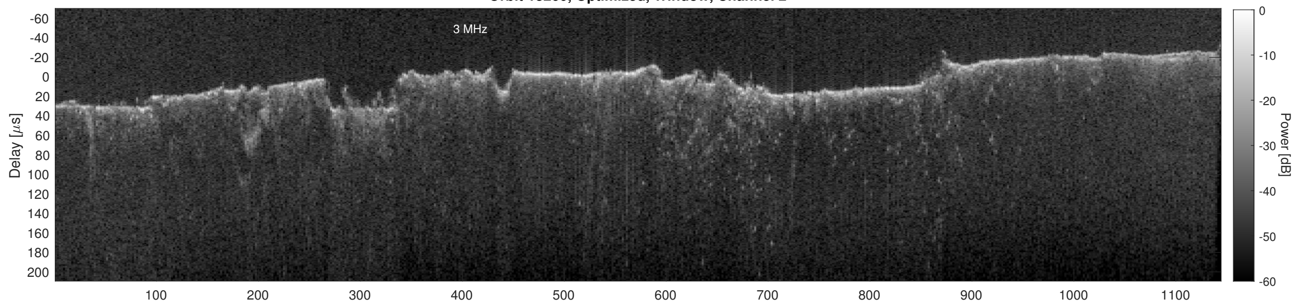
Orbit 13260, Cluttergram
