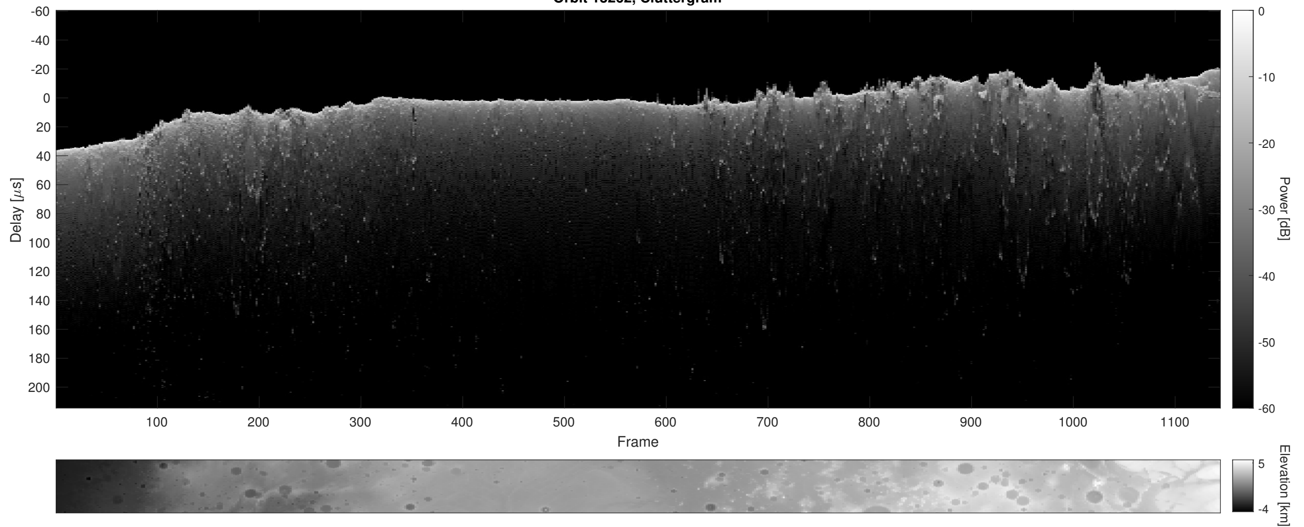
Orbit 13262, Cluttergram
