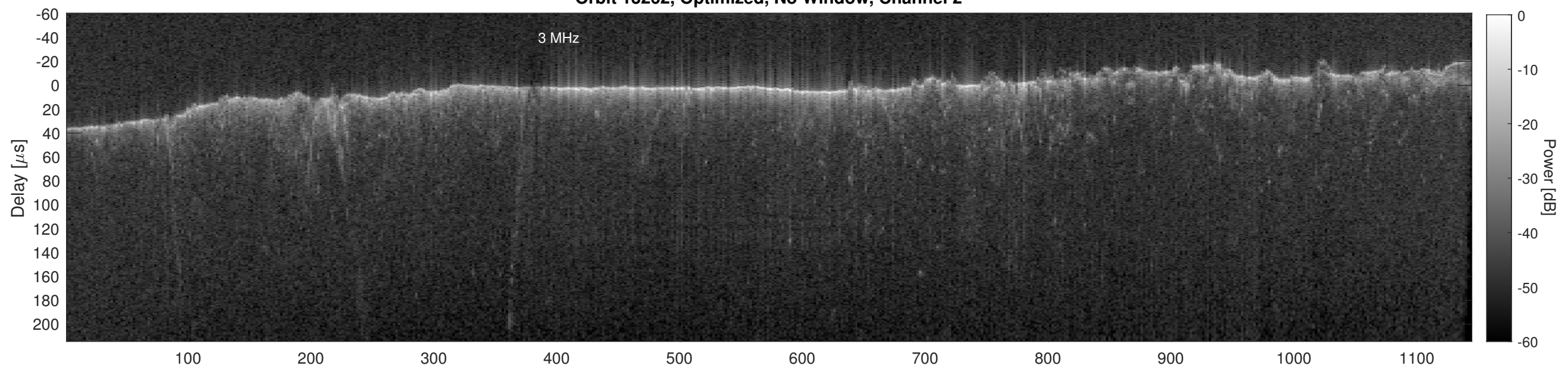
Orbit 13262, Cluttergram
