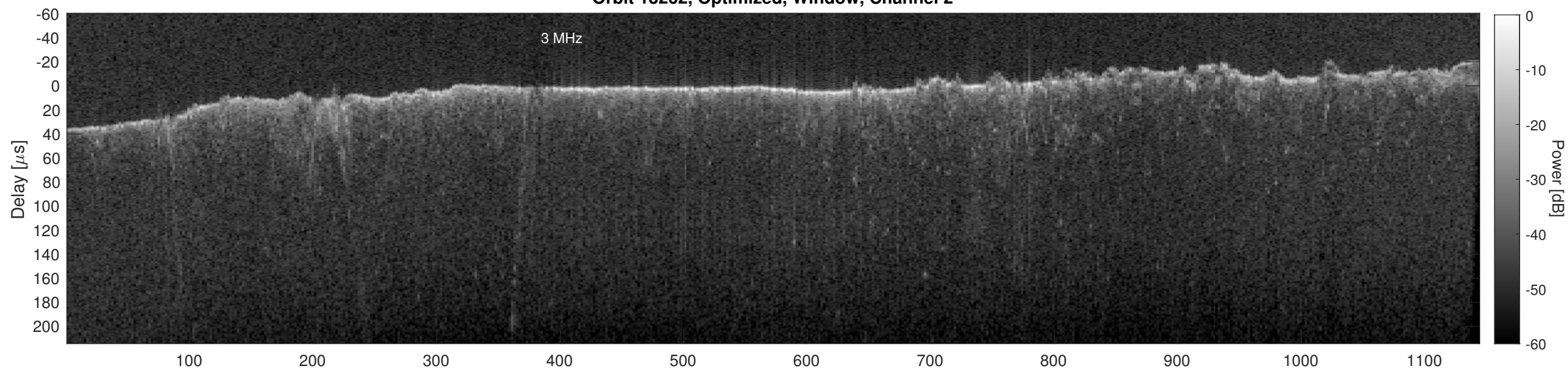
Orbit 13262, Cluttergram
