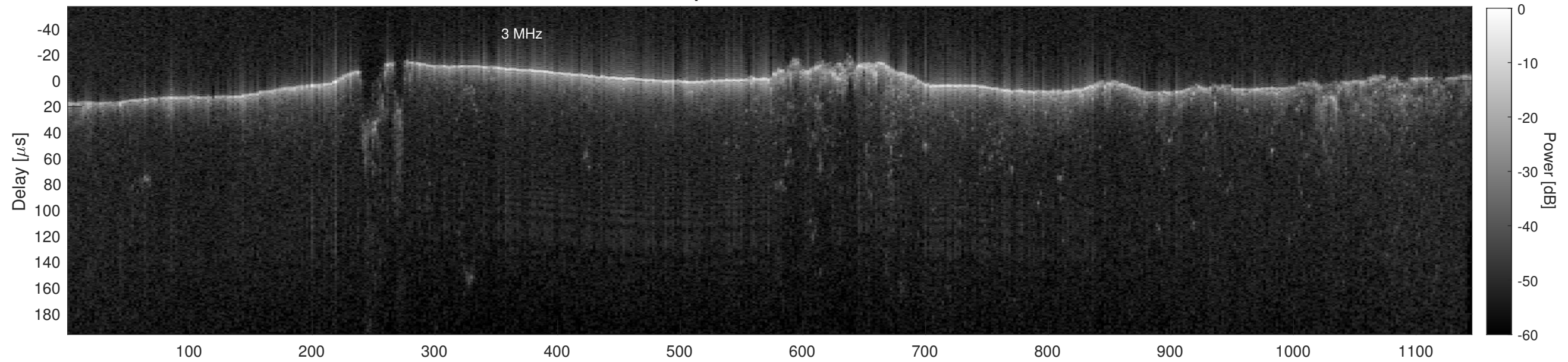
Orbit 13264, Cluttergram
