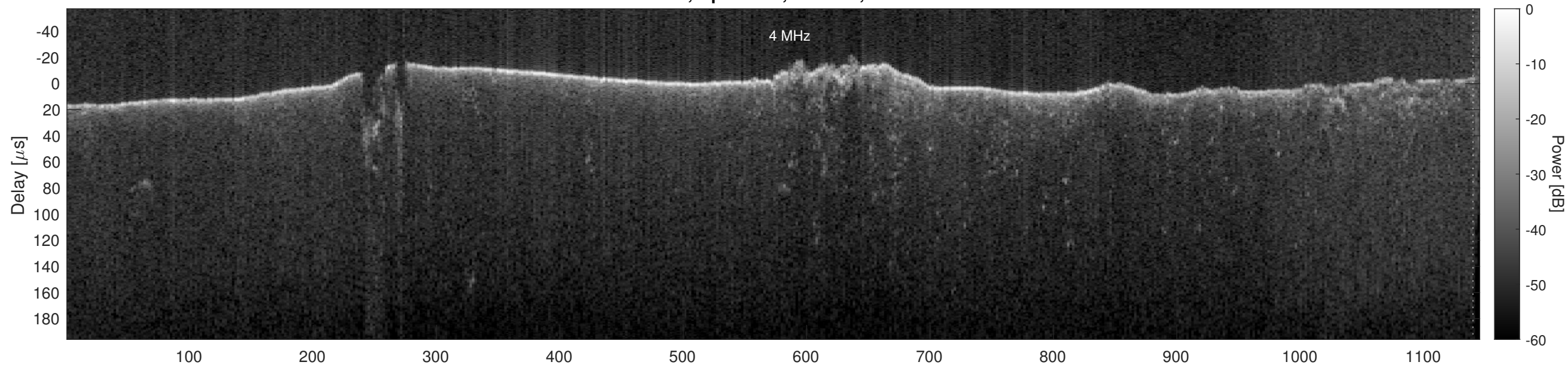
Orbit 13264, Optimized, Window, Channel 2
