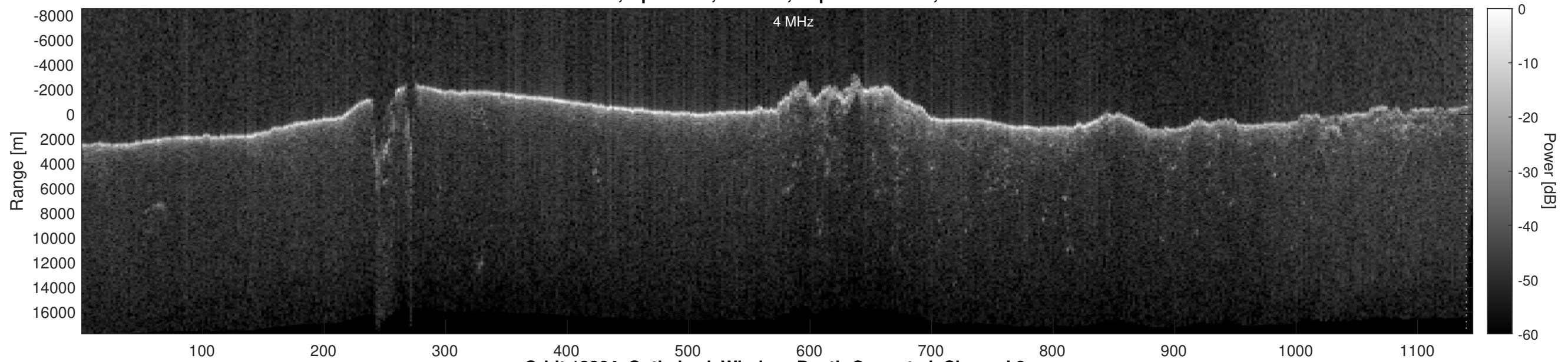
Orbit 13264, Optimized, Window, Depth-Corrected, Channel 2
