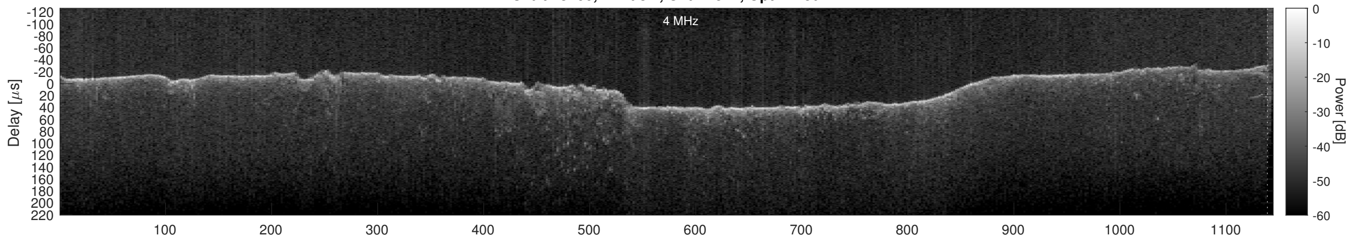
Orbit 13266, Cluttergram
